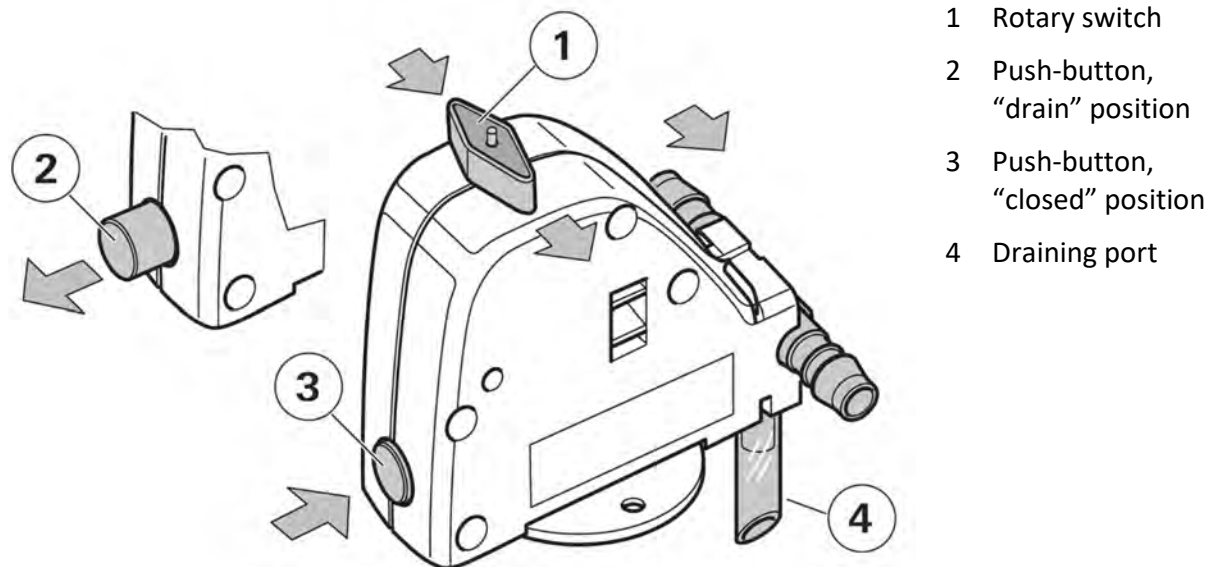
"FrostControl" drain valve
