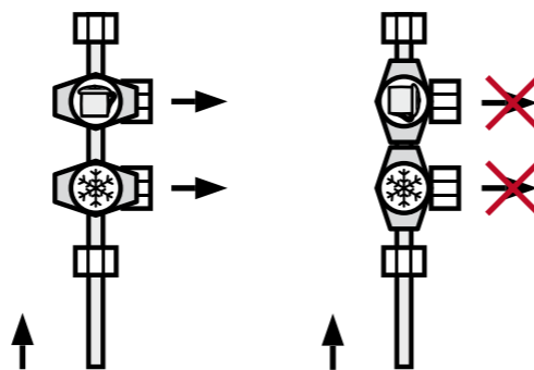
Stopcock open
